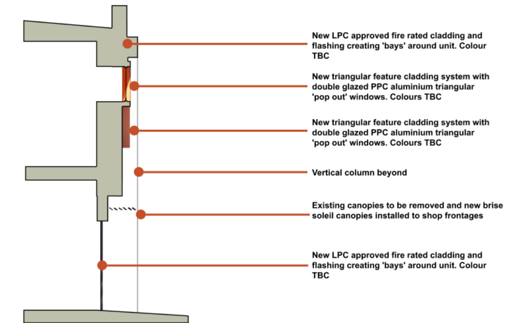
Typical 'Bay' Section
